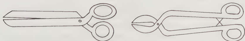
Figure 20.1 Which shear would be better for cutting metal?
