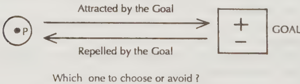
Figure 13.11 Approach-avoidance conflict.
